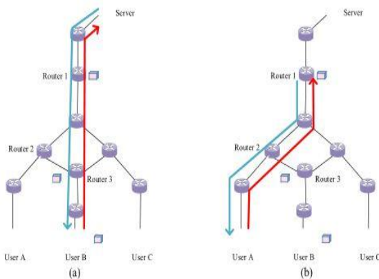
Fig. 1 Problem analysis of on-path caching.
