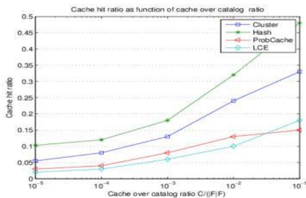
Fig. 9 cache hit ratio as function of cache over catalog ratio
