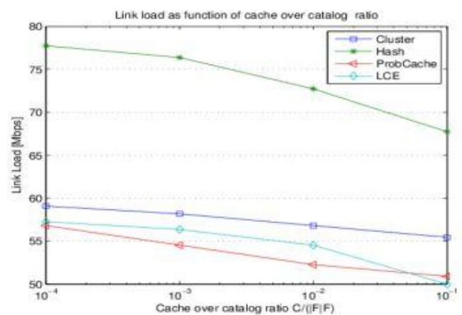
Fig. 11 Link load as function of cache over catalog ratio
