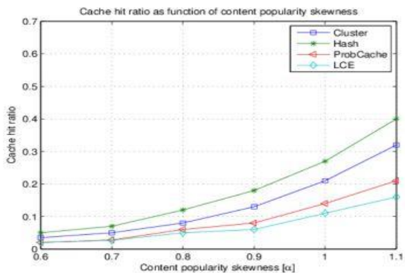
Fig. 10 Cache hit ratio as function of content popularity skewness
