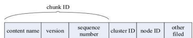
Fig. 7 An example of Interest packet
