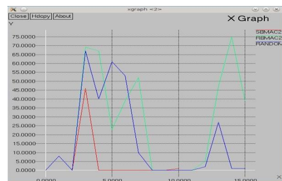
Fig5.Throughput Second scenario
