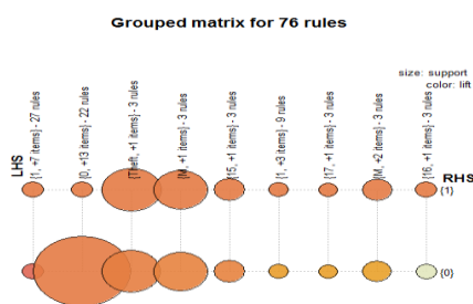
Figure 3.3. Group Matrix
