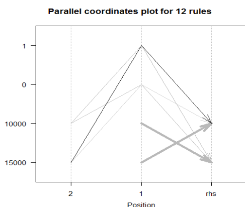
Figure 2.3: Parallel Coordination.
