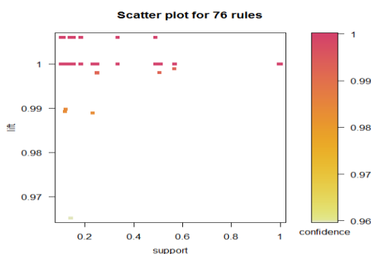
Figure 3.4: Scatter Plot
