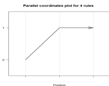
Figure 2.3: Parallel Coordination.
