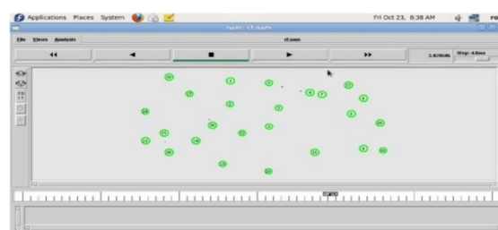
Fig 3 Node Initialization
