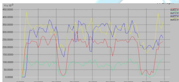
Fig. 6. AOMDV without network security breaches
