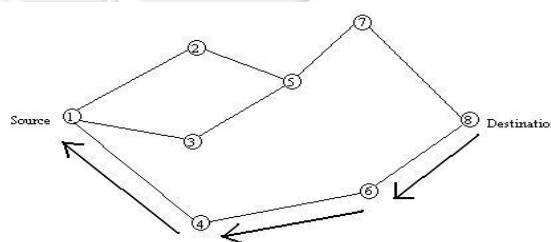
Fig. 2. Path taken by the Route Reply Packet
