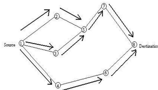
Fig. 1. Propagation of Route Request Packet
