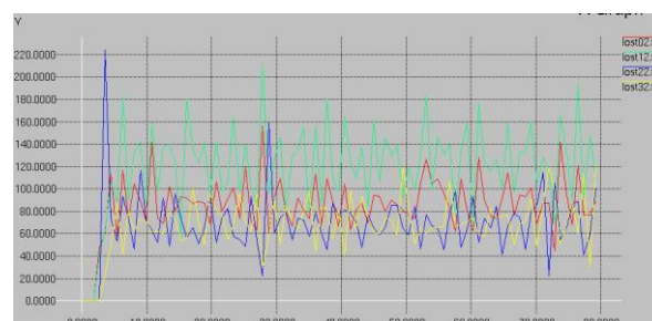
Fig. 10. AOMDV packet loss without network security
