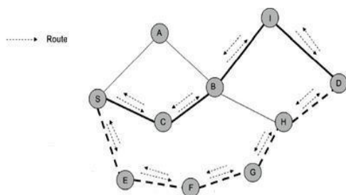
Fig. 3. AOMDV route discovery
